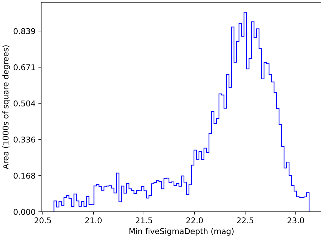
ddf_half_v3.4_10yrs Yr 1 z band: Min fiveSigmaDepth
