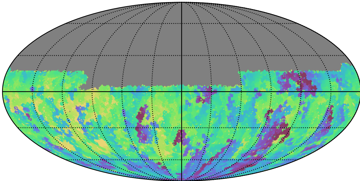
ddf_half_v3.4_10yrs Yr 1 u band: Min fiveSigmaDepth
