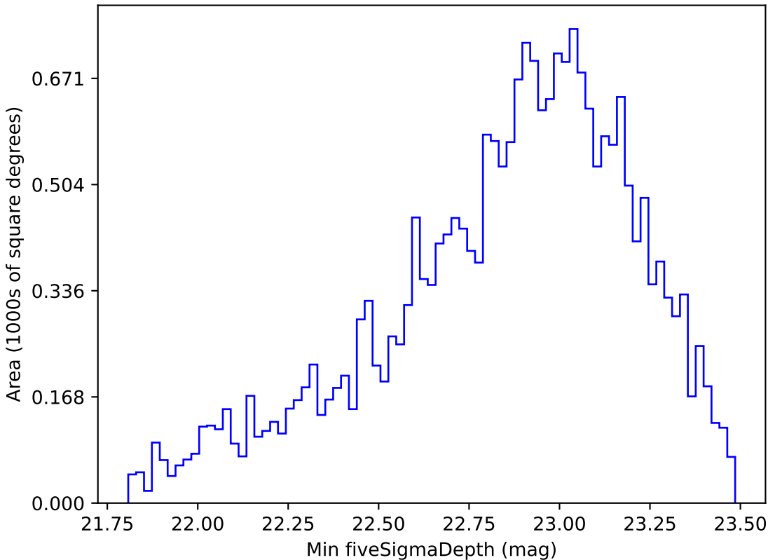
ddf_half_v3.4_10yrs Yr 1 u band: Min fiveSigmaDepth
