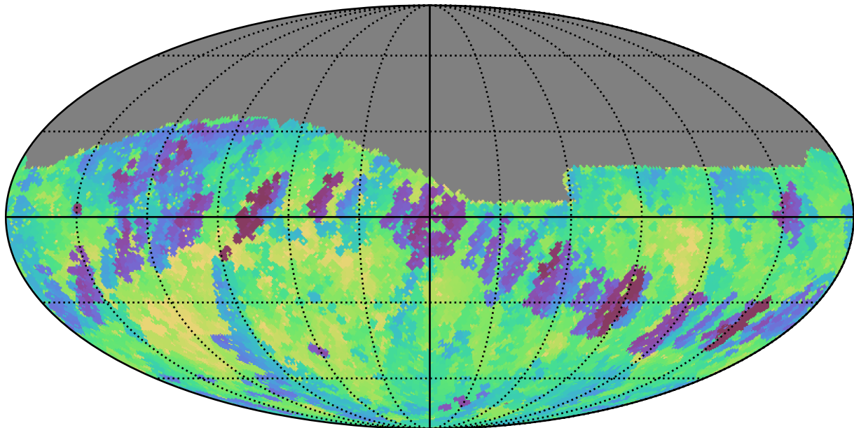
ddf_half_v3.4_10yrs Yr 1 r band: Min fiveSigmaDepth
