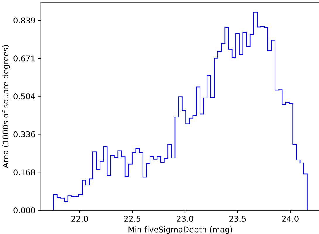
ddf_half_v3.4_10yrs Yr 1 r band: Min fiveSigmaDepth
