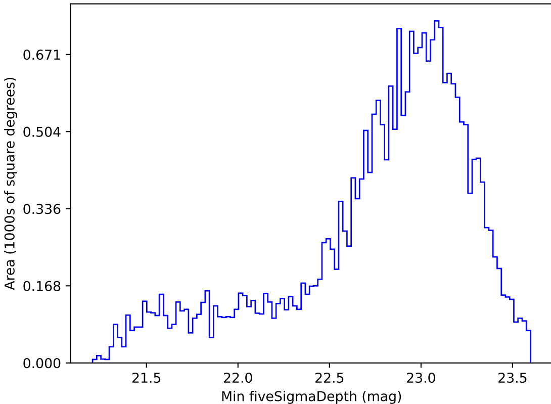
ddf_half_v3.4_10yrs Yr 1 i band: Min fiveSigmaDepth
