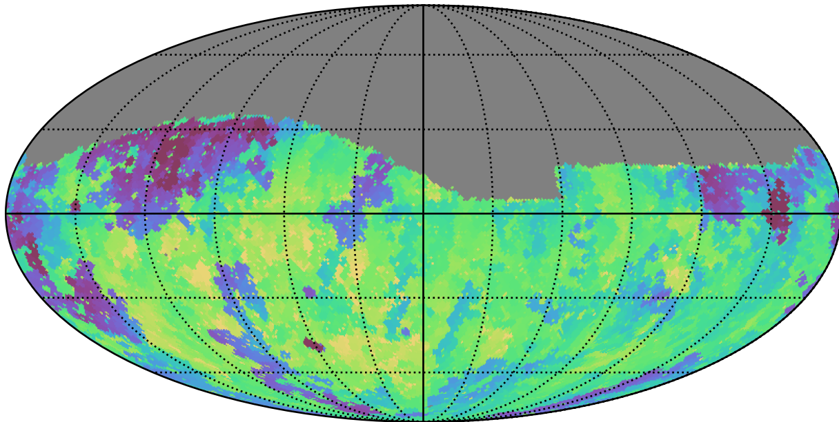
ddf_half_v3.4_10yrs Yr 1 g band: Min fiveSigmaDepth
