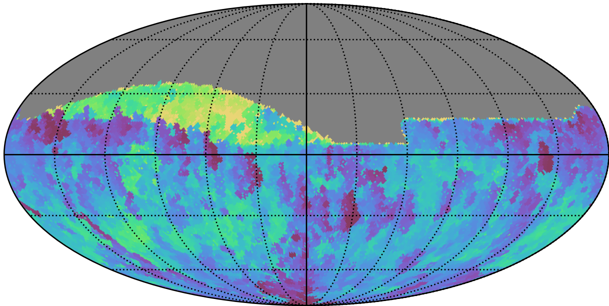
ddf_half_v3.4_10yrs Yr 1 all bands: Min fiveSigmaDepth
