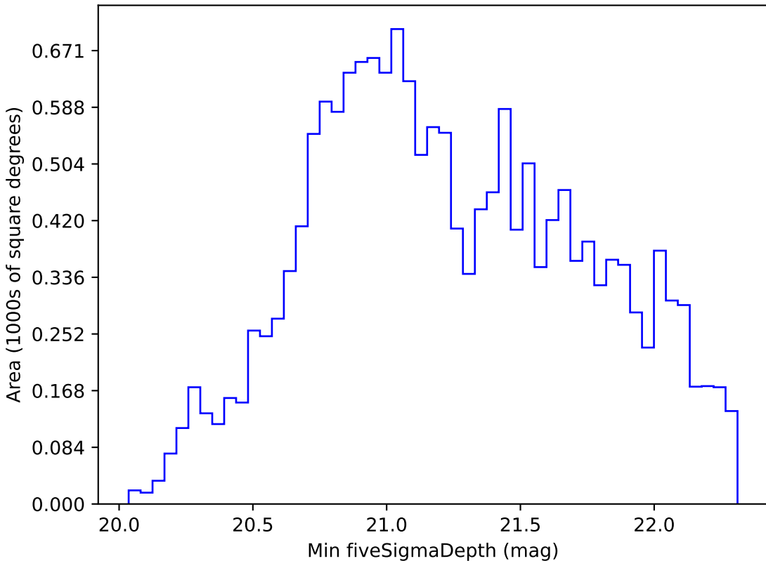
ddf_half_v3.4_10yrs WFD z band: Min fiveSigmaDepth
