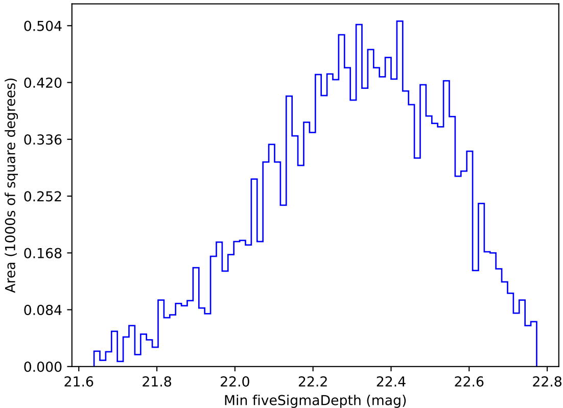
ddf_half_v3.4_10yrs WFD u band: Min fiveSigmaDepth
