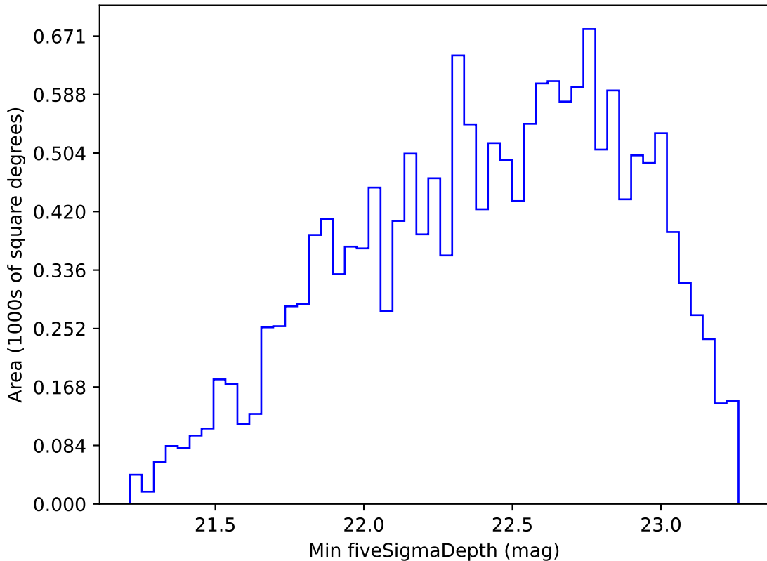
ddf_half_v3.4_10yrs WFD r band: Min fiveSigmaDepth
