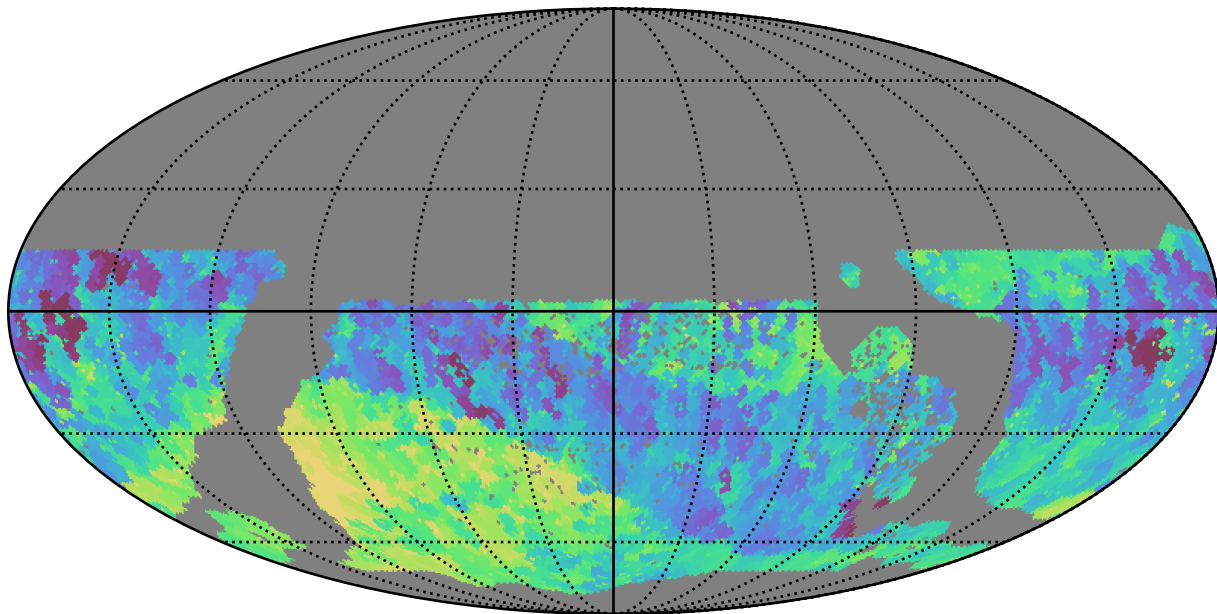
ddf_half_v3.4_10yrs WFD i band: Min fiveSigmaDepth
