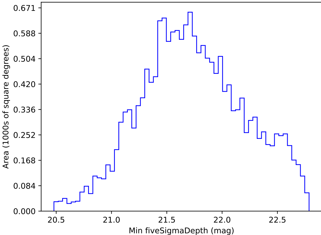
ddf_half_v3.4_10yrs WFD i band: Min fiveSigmaDepth
