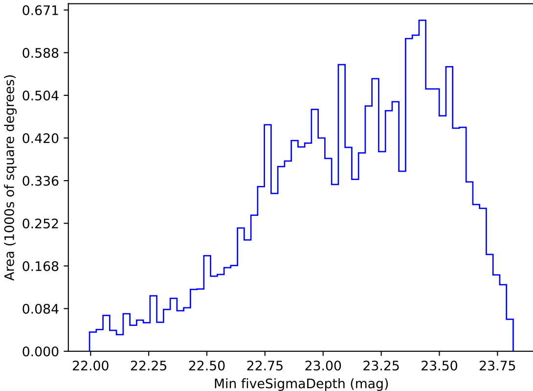
ddf_half_v3.4_10yrs WFD g band: Min fiveSigmaDepth
