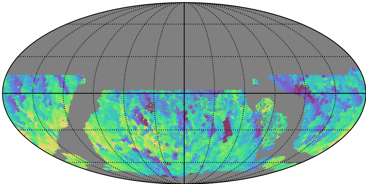
ddf_half_v3.4_10yrs WFD all bands: Min fiveSigmaDepth
