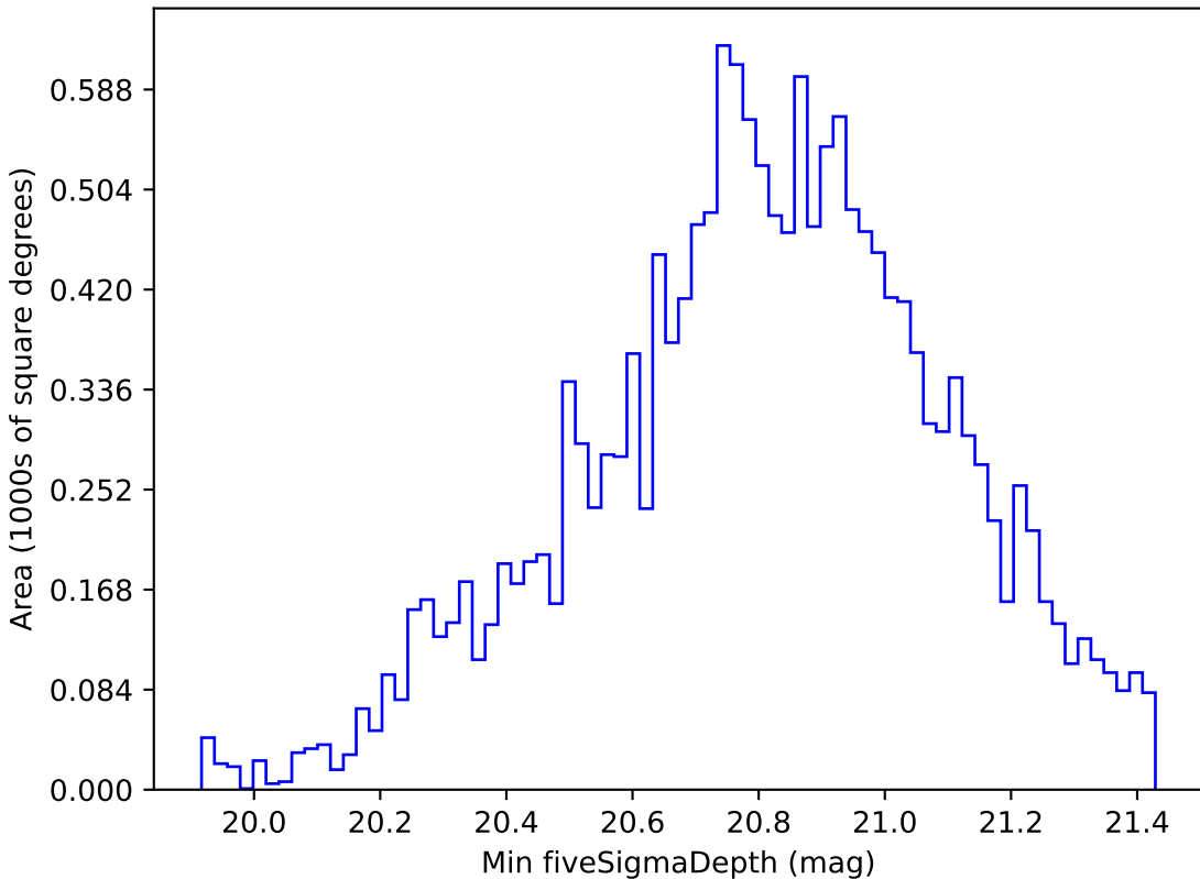
ddf_half_v3.4_10yrs WFD all bands: Min fiveSigmaDepth
