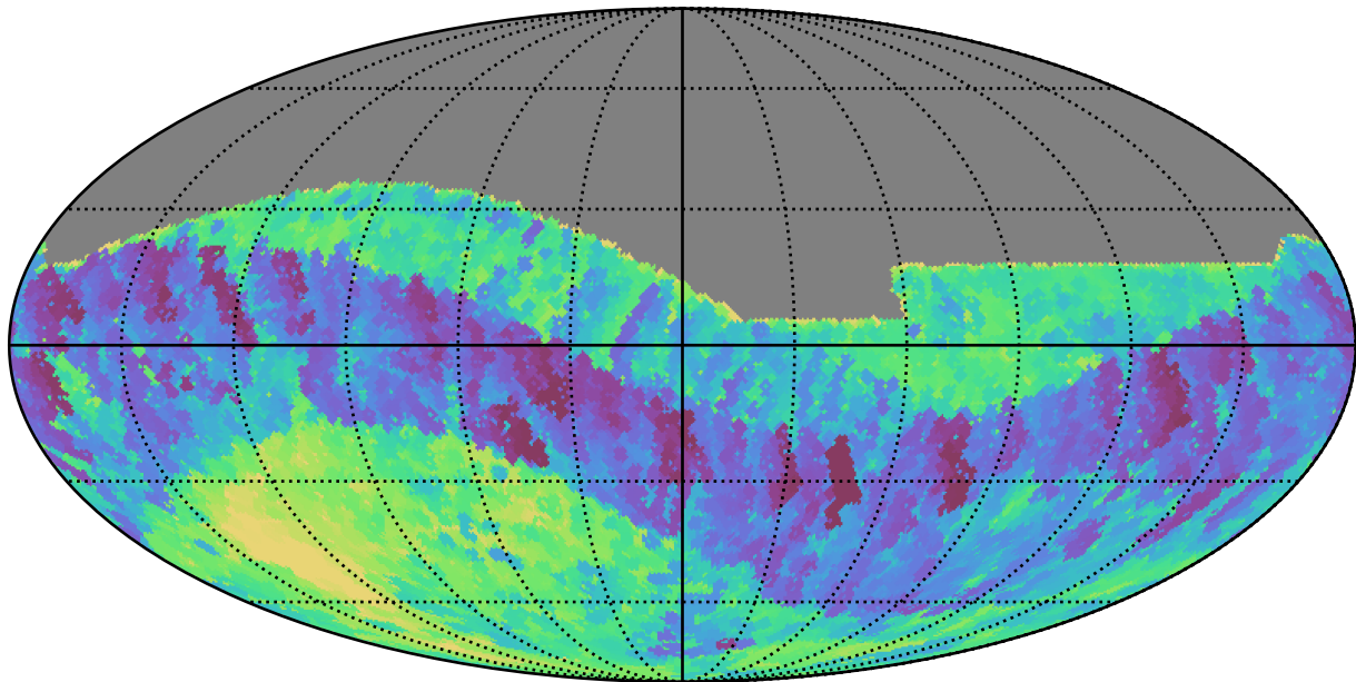
ddf_half_v3.4_10yrs All sky z band: Min fiveSigmaDepth
