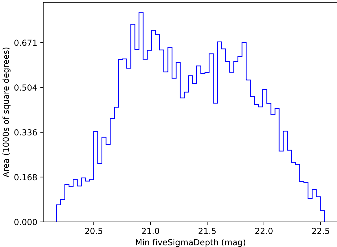
ddf_half_v3.4_10yrs All sky z band: Min fiveSigmaDepth
