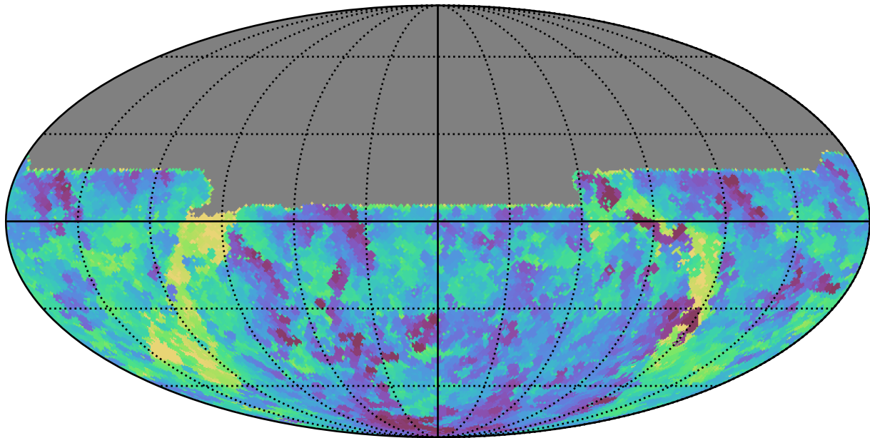
ddf_half_v3.4_10yrs All sky u band: Min fiveSigmaDepth
