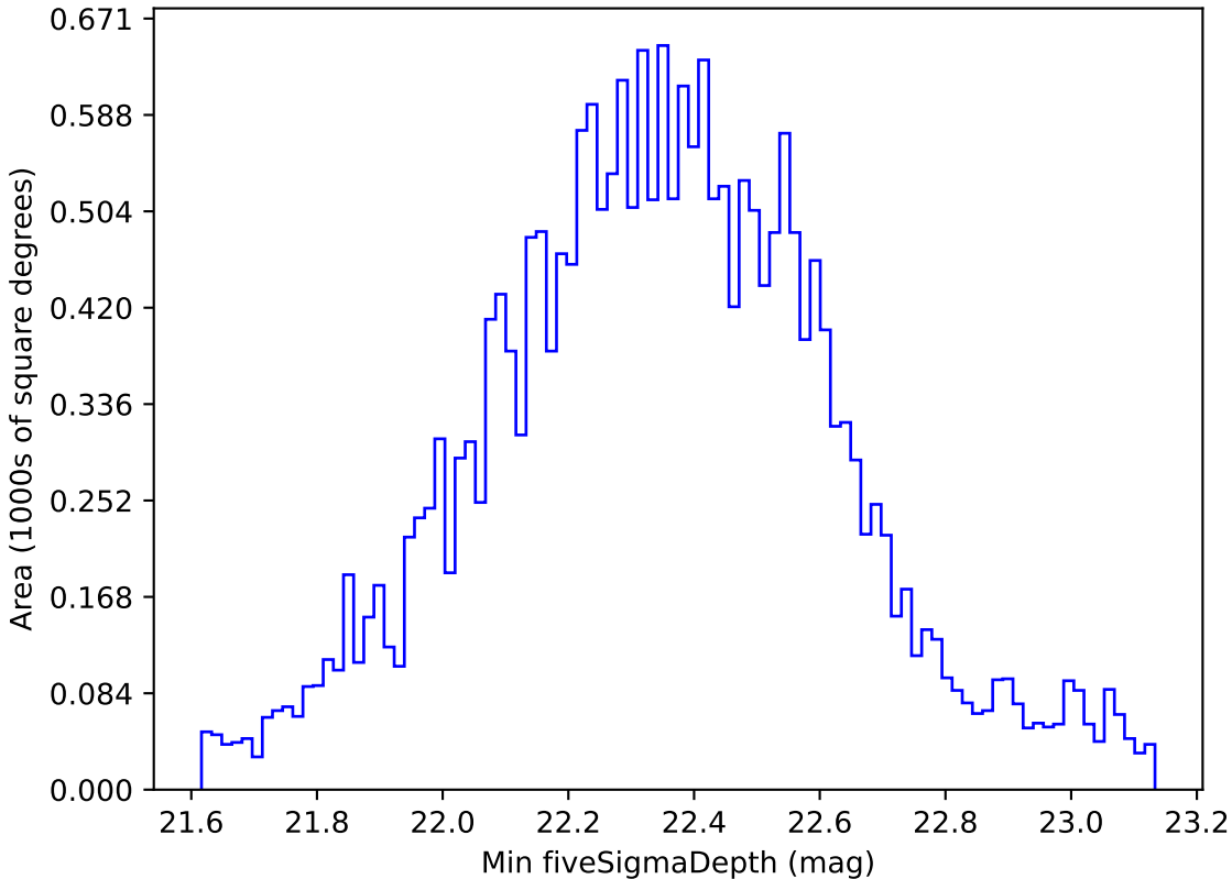
ddf_half_v3.4_10yrs All sky u band: Min fiveSigmaDepth
