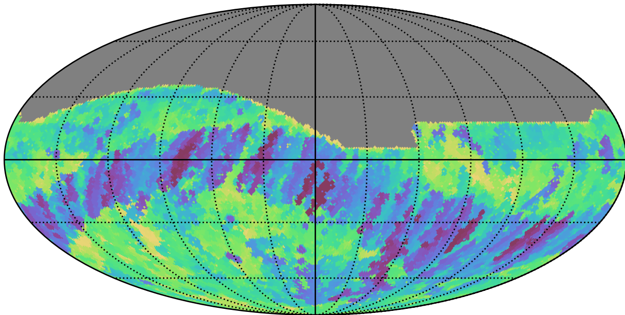
ddf_half_v3.4_10yrs All sky r band: Min fiveSigmaDepth
