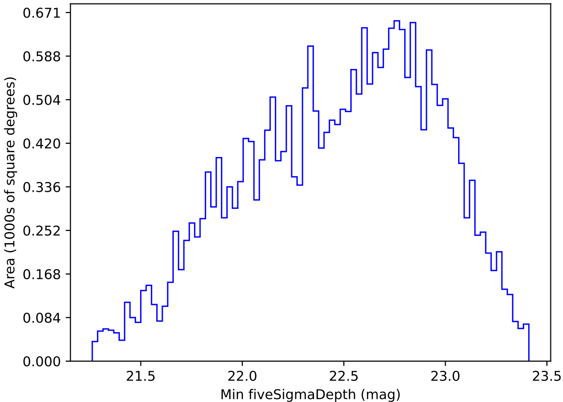
ddf_half_v3.4_10yrs All sky r band: Min fiveSigmaDepth
