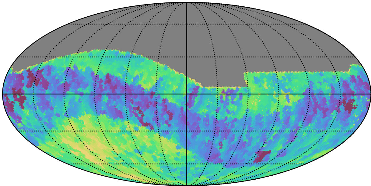
ddf_half_v3.4_10yrs All sky i band: Min fiveSigmaDepth
