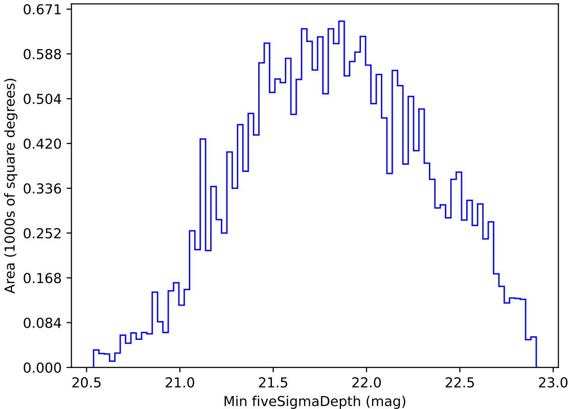
ddf_half_v3.4_10yrs All sky i band: Min fiveSigmaDepth
