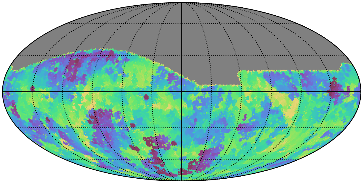
ddf_half_v3.4_10yrs All sky g band: Min fiveSigmaDepth
