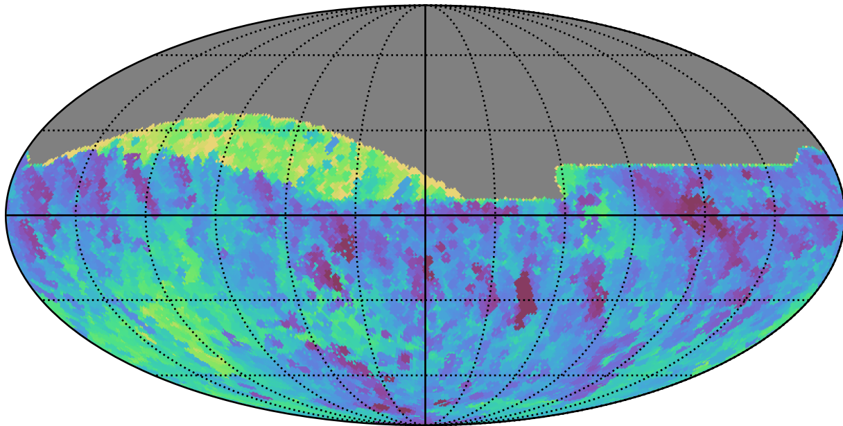
ddf_half_v3.4_10yrs All sky all bands: Min fiveSigmaDepth
