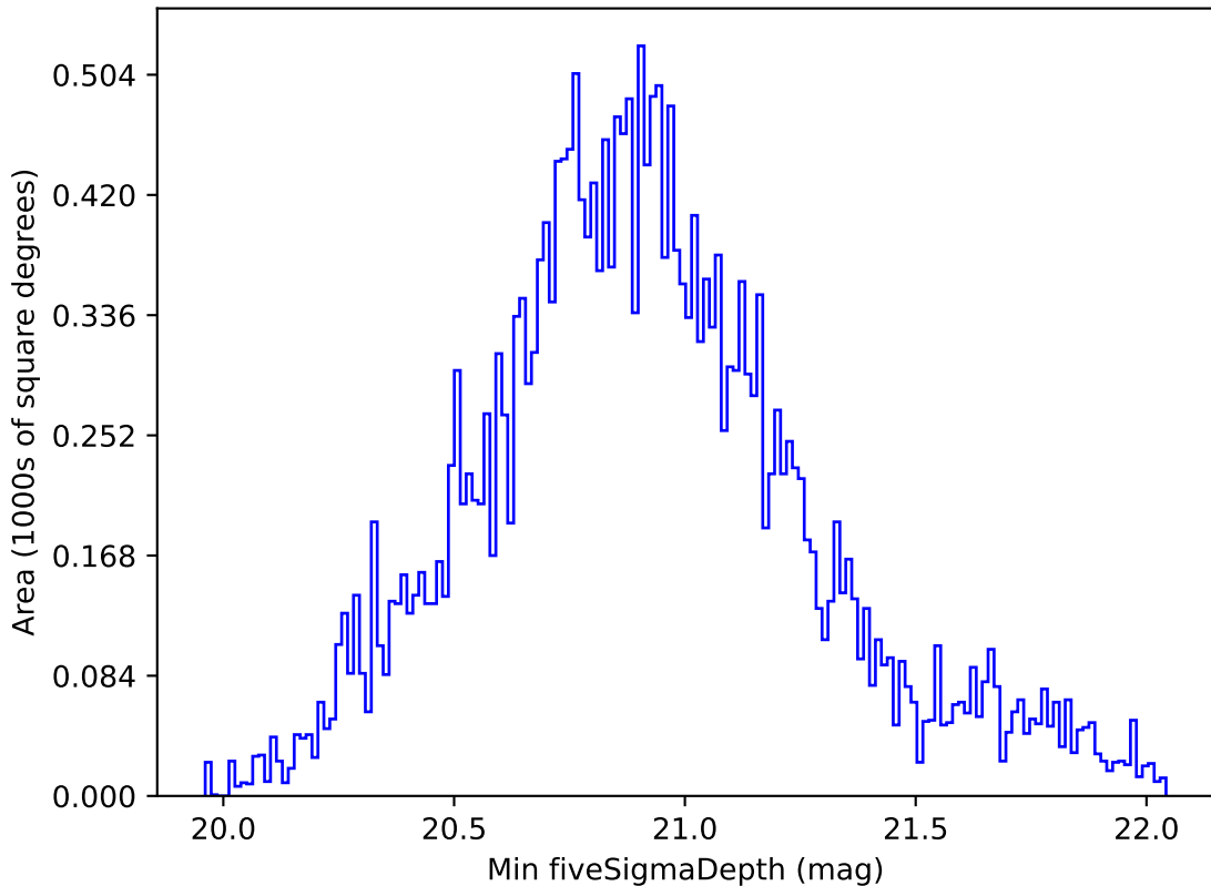
ddf_half_v3.4_10yrs All sky all bands: Min fiveSigmaDepth
