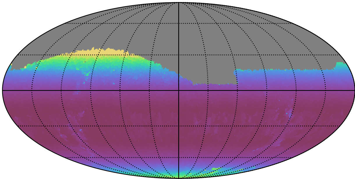
ddf_half_v3.4_10yrs Yr 1 z band: Min airmass
