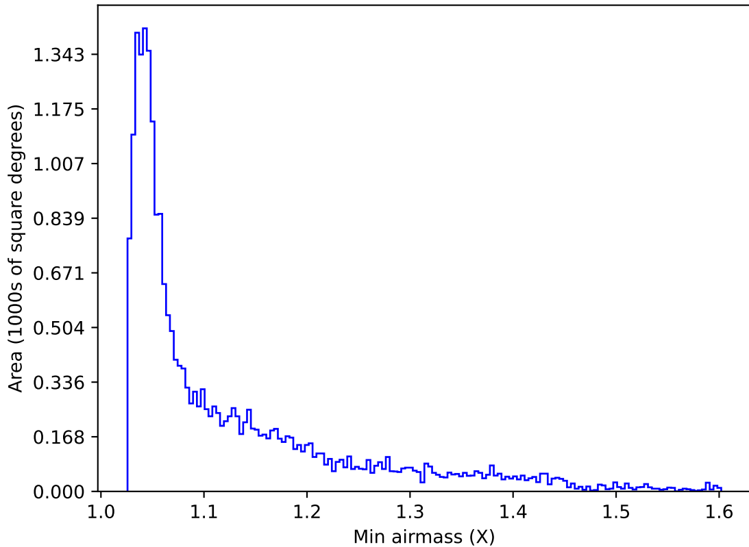
ddf_half_v3.4_10yrs Yr 1 y band: Min airmass
