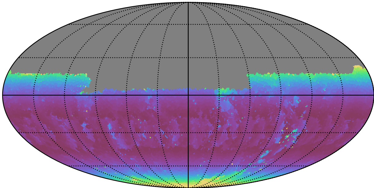
ddf_half_v3.4_10yrs Yr 1 u band: Min airmass
