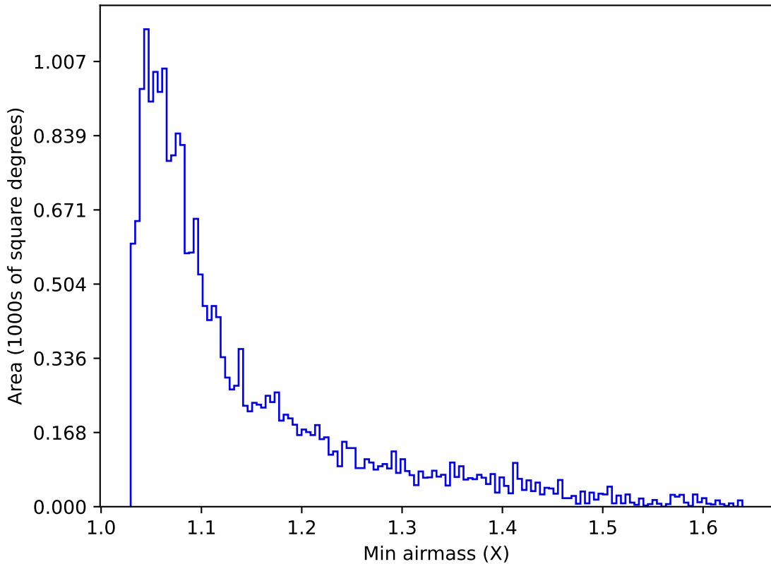
ddf_half_v3.4_10yrs Yr 1 u band: Min airmass
