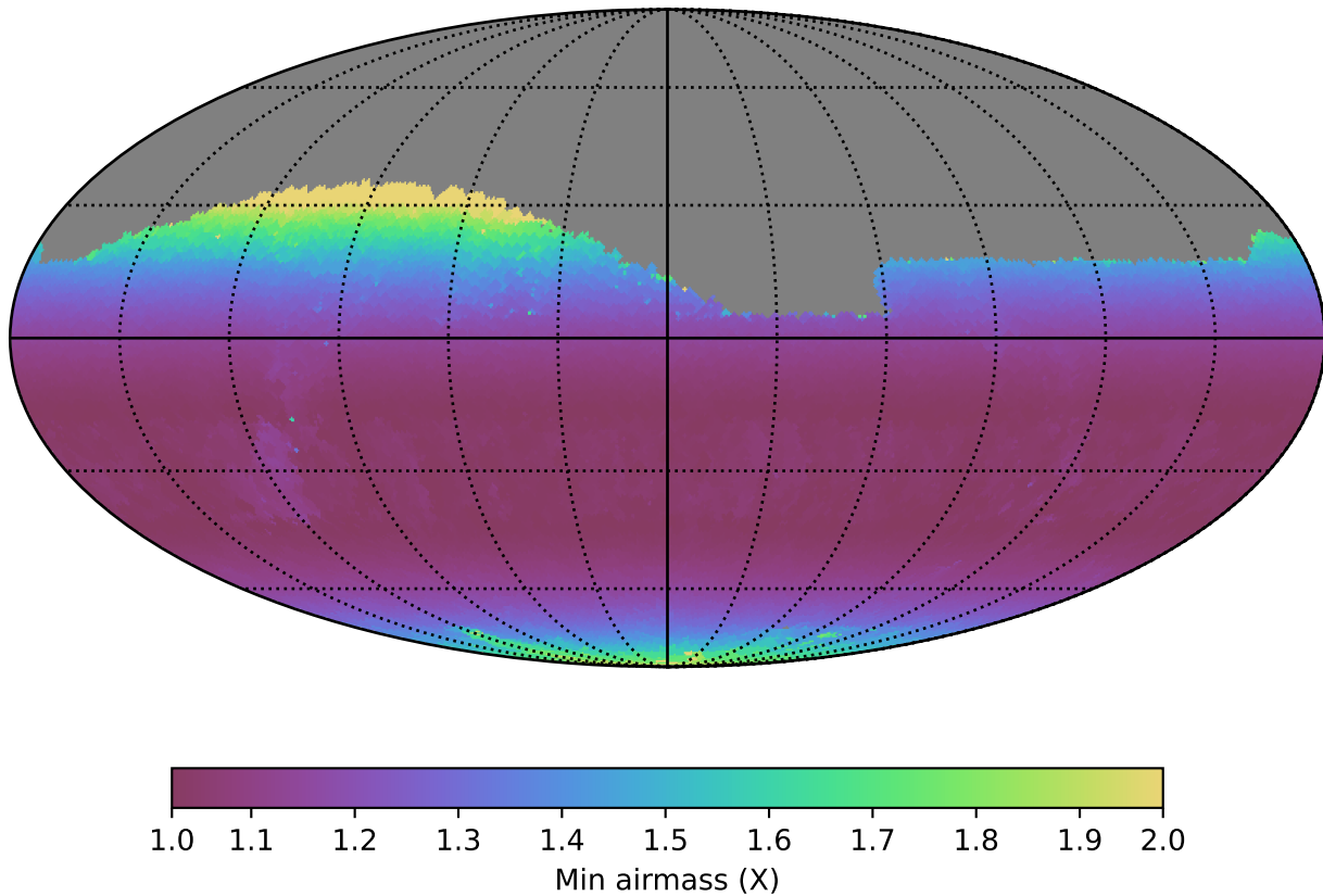
ddf_half_v3.4_10yrs Yr 1 r band: Min airmass
