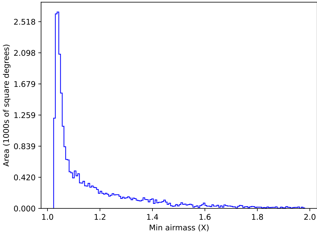
ddf_half_v3.4_10yrs Yr 1 r band: Min airmass
