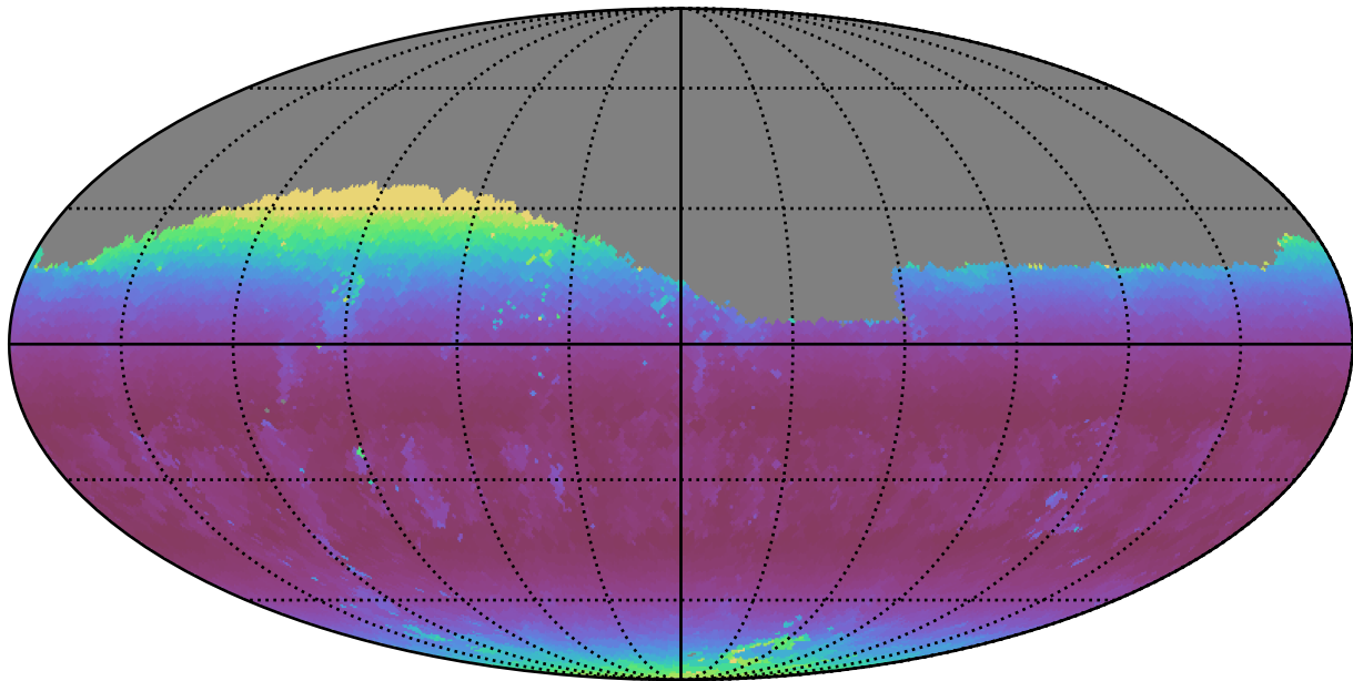
ddf_half_v3.4_10yrs Yr 1 g band: Min airmass
