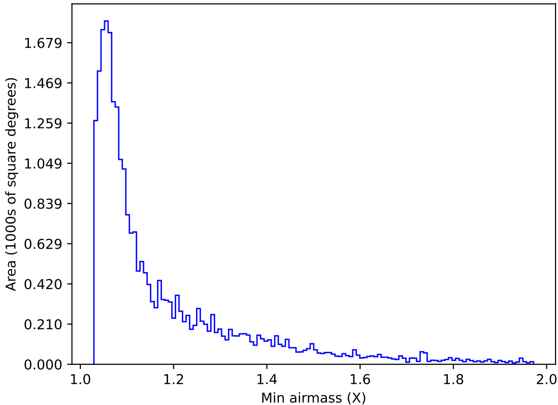
ddf_half_v3.4_10yrs Yr 1 g band: Min airmass
