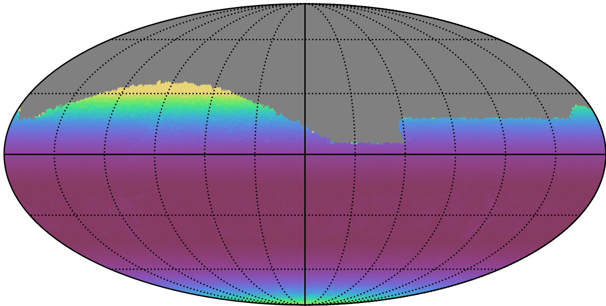
ddf_half_v3.4_10yrs Yr 1 all bands: Min airmass
