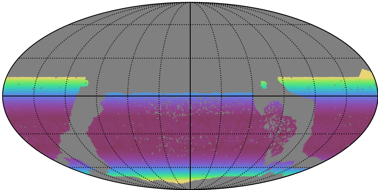
ddf_half_v3.4_10yrs WFD z band: Min airmass
