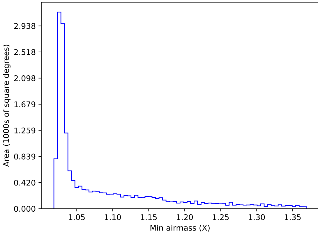
ddf_half_v3.4_10yrs WFD z band: Min airmass
