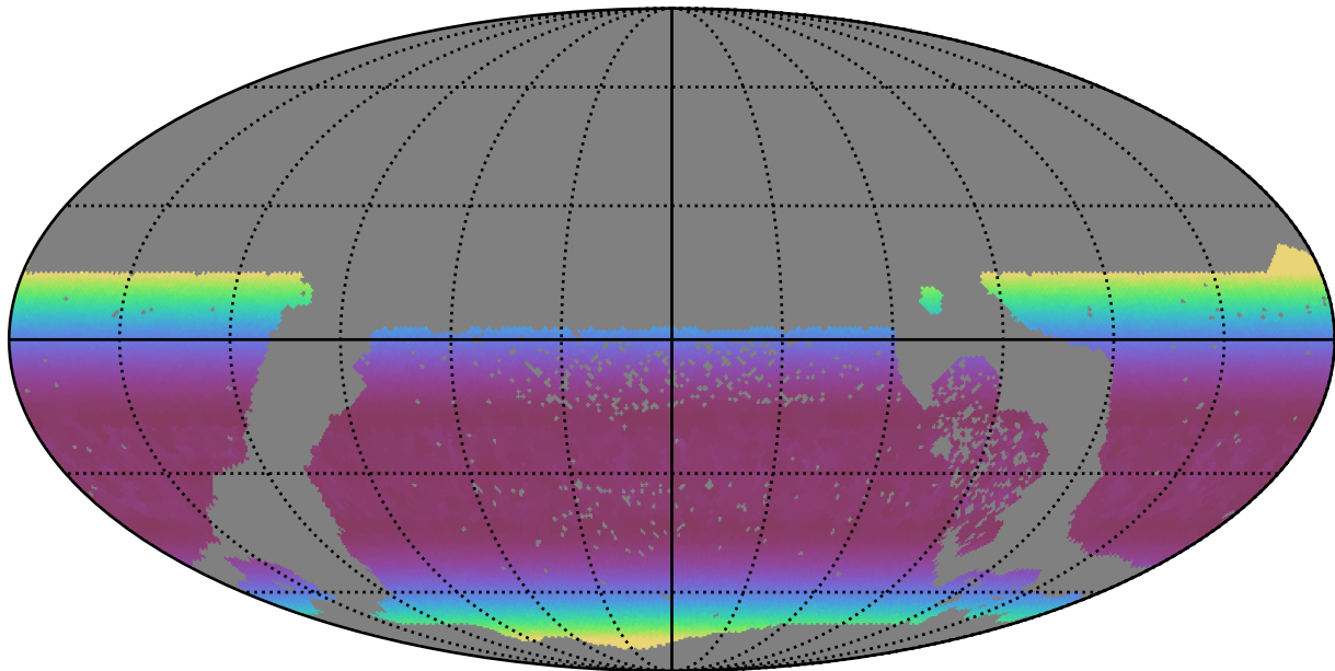
ddf_half_v3.4_10yrs WFD y band: Min airmass
