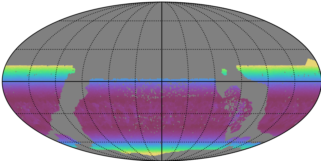
ddf_half_v3.4_10yrs WFD u band: Min airmass
