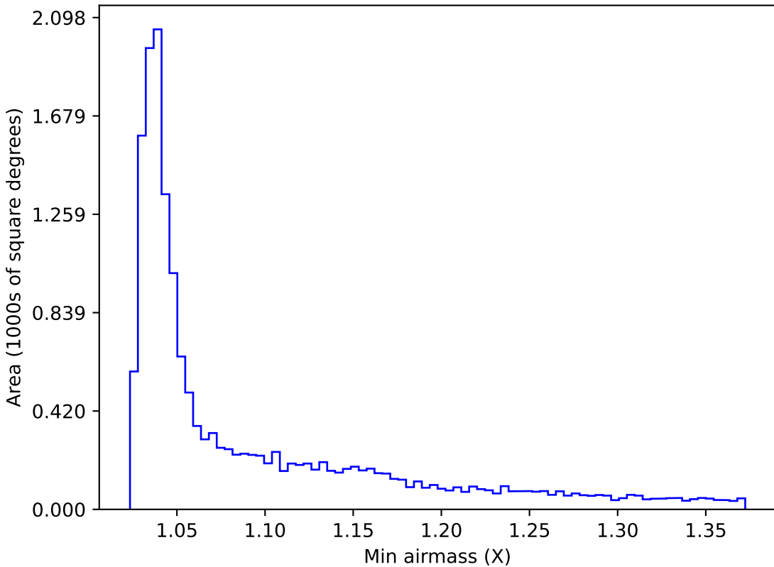
ddf_half_v3.4_10yrs WFD u band: Min airmass
