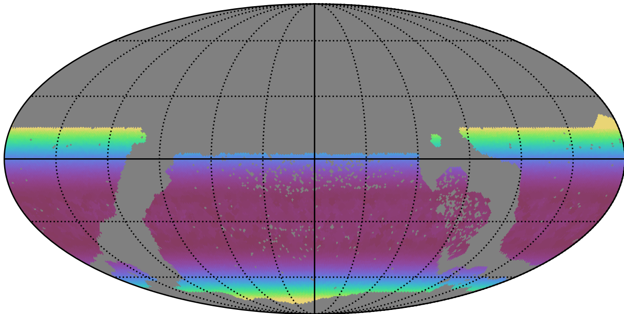
ddf_half_v3.4_10yrs WFD r band: Min airmass
