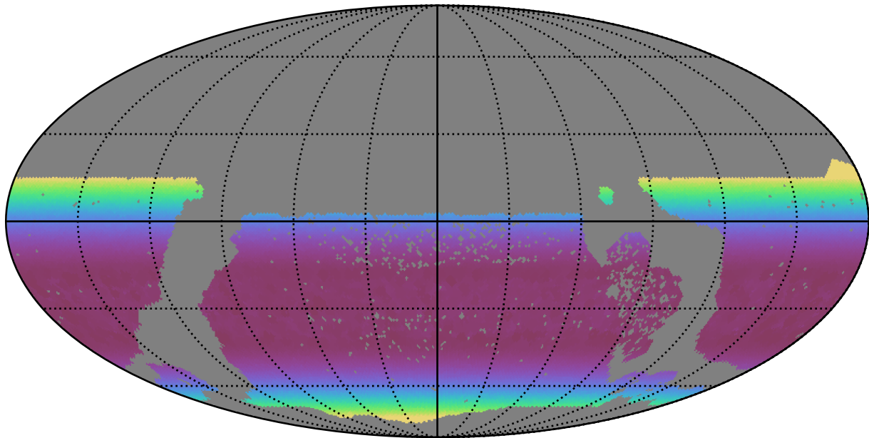
ddf_half_v3.4_10yrs WFD i band: Min airmass
