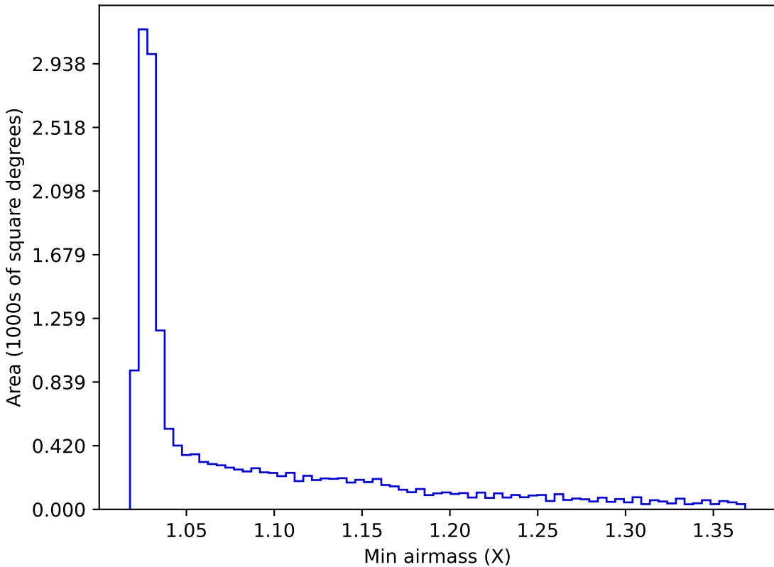
ddf_half_v3.4_10yrs WFD i band: Min airmass
