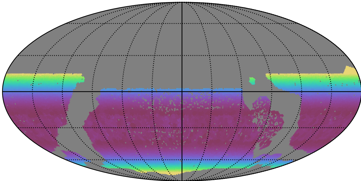
ddf_half_v3.4_10yrs WFD g band: Min airmass
