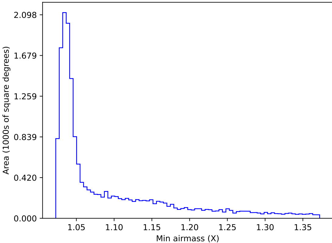
ddf_half_v3.4_10yrs WFD g band: Min airmass
