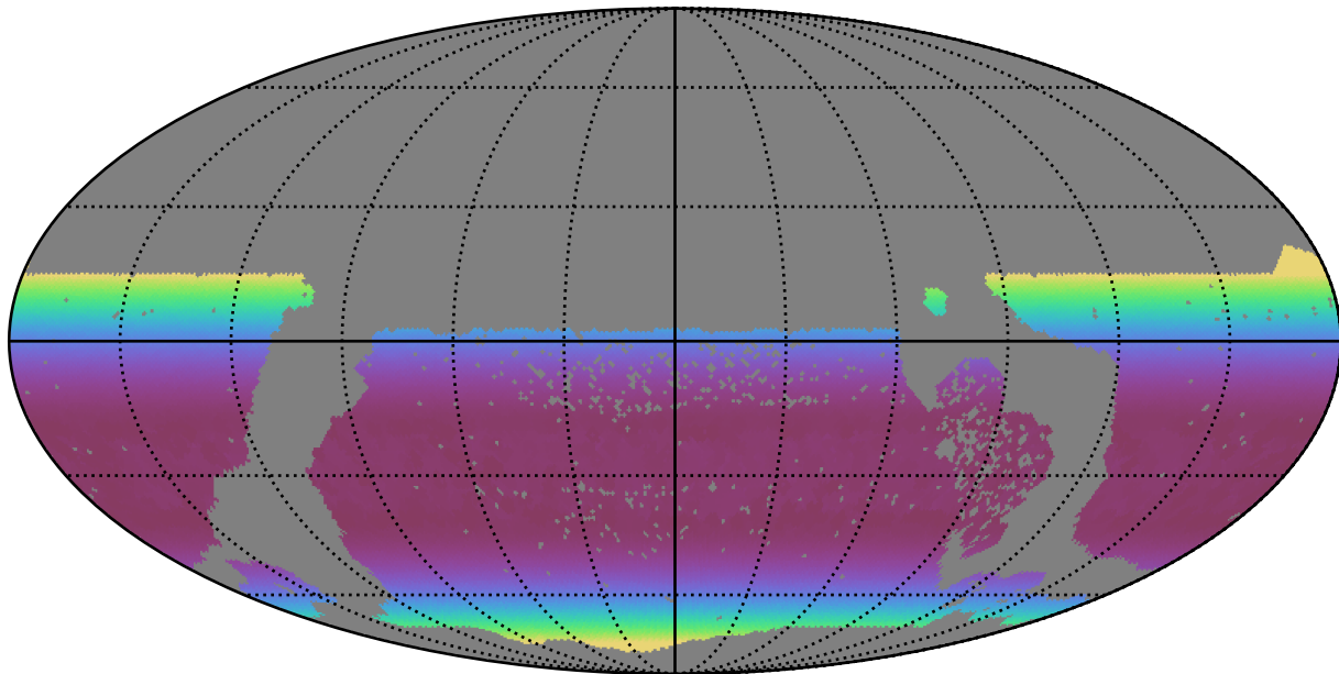
ddf_half_v3.4_10yrs WFD all bands: Min airmass
