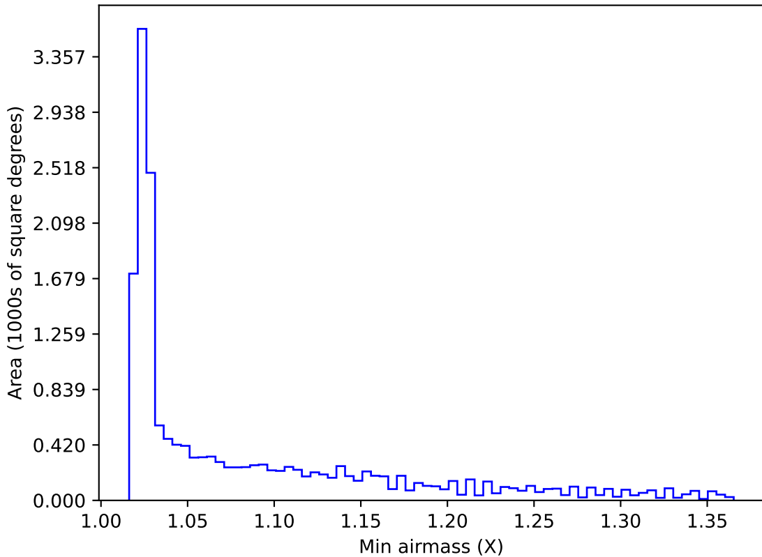
ddf_half_v3.4_10yrs WFD all bands: Min airmass
