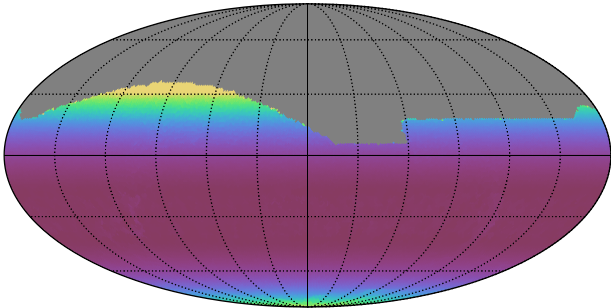
ddf_half_v3.4_10yrs All sky z band: Min airmass
