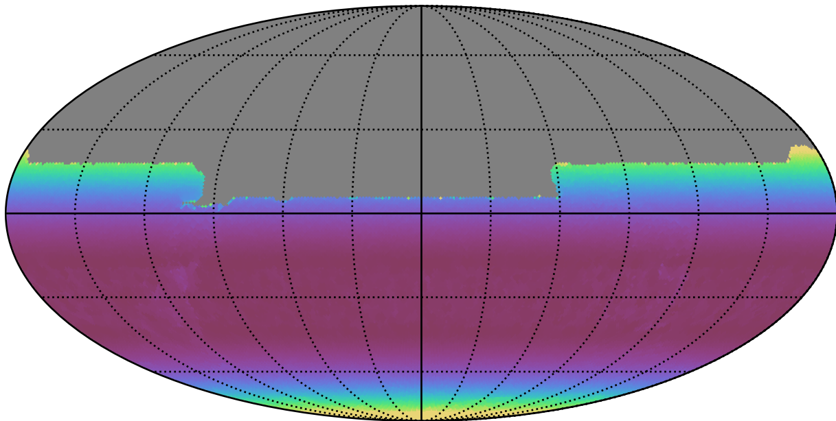
ddf_half_v3.4_10yrs All sky y band: Min airmass
